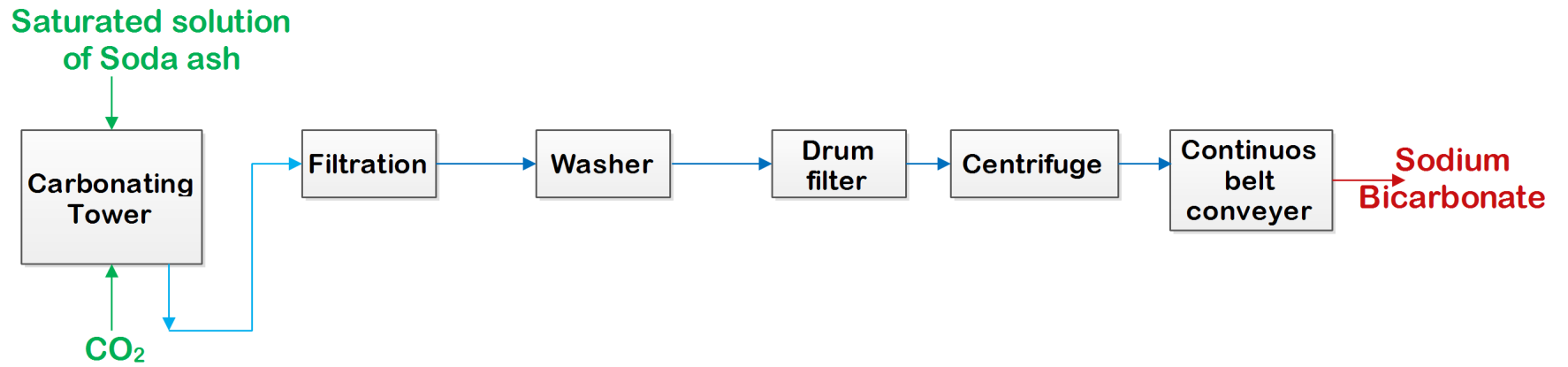
Figure: Manufacturing of Sodium Bicarbonate
